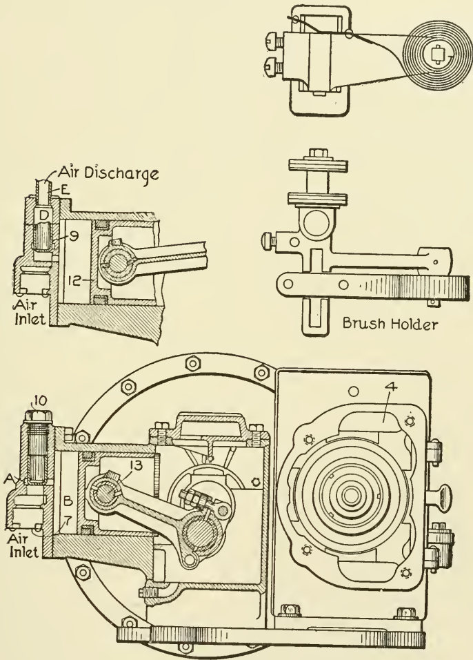
Fig. 86. Diagram of Parts of Motor Driven from Pressure
